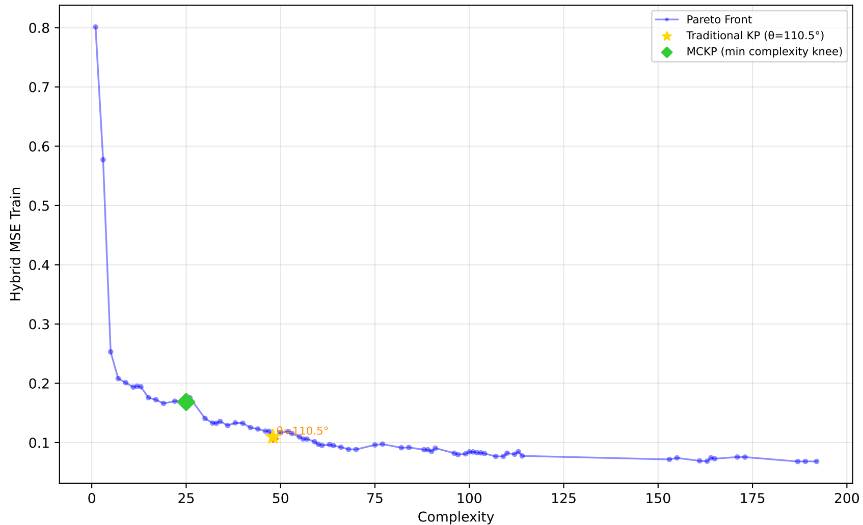
1096_FacultySalaries - Run 12 - SVP - Hybrid MSE Train \lambda_1=1.00 , \lambda_2=0.00 , \lambda_3=0.00 | Difficulty: 1.00 | Method: hmr
