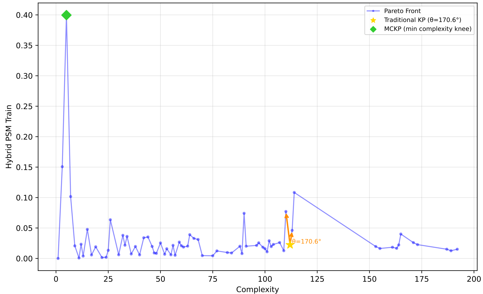
1096_FacultySalaries - Run 12 - SVP - Hybrid PSM Train \lambda_1=0.00 , \lambda_2=0.90 , \lambda_3=0.00 | Difficulty: 1.00 | Method: hmr
