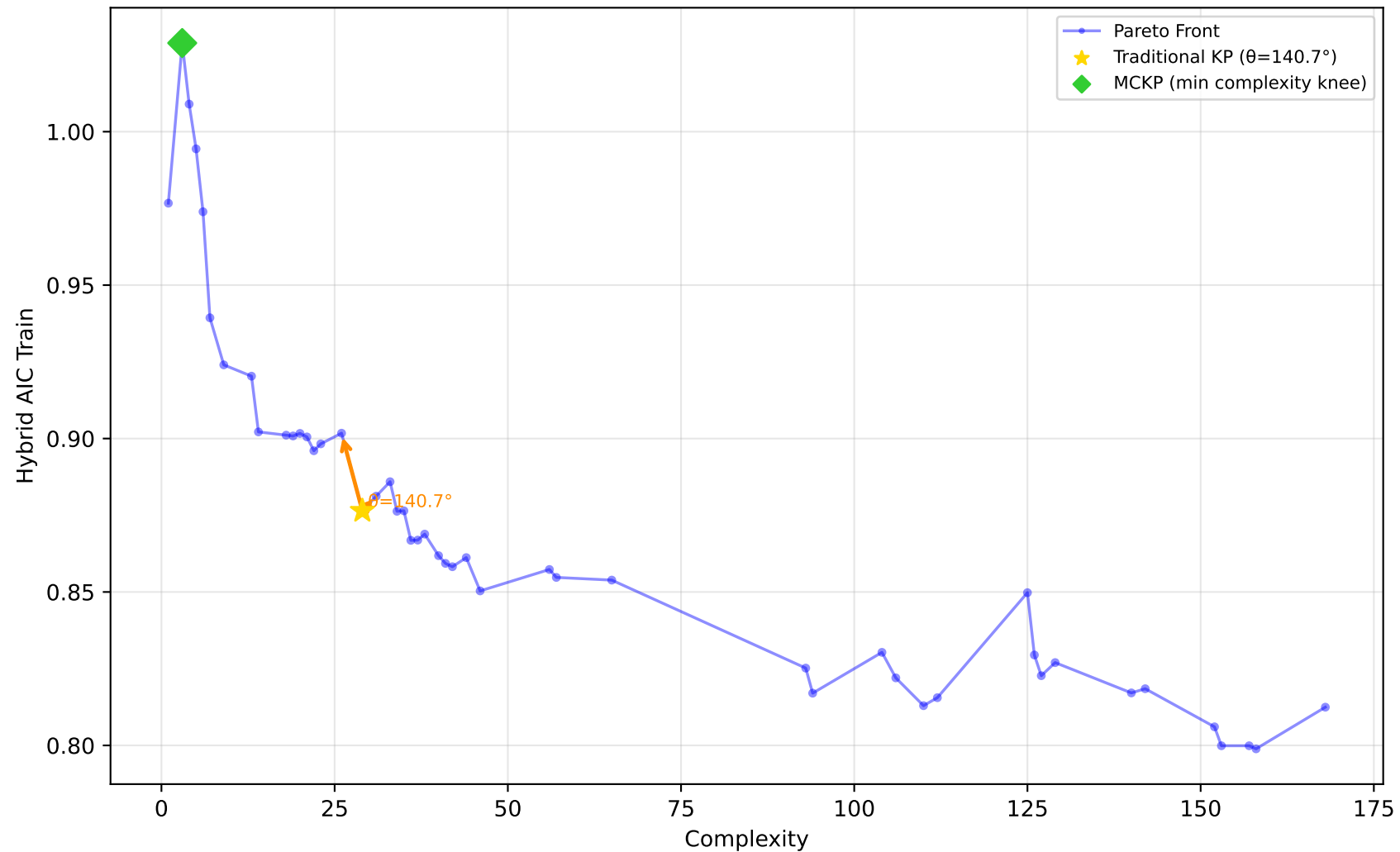
1096_FacultySalaries - Run 13 - MVP - Hybrid AIC Train \lambda_1=1.00 , \lambda_2=0.00 , \lambda_3=0.00 | Difficulty: 1.00 | Method: hmr
