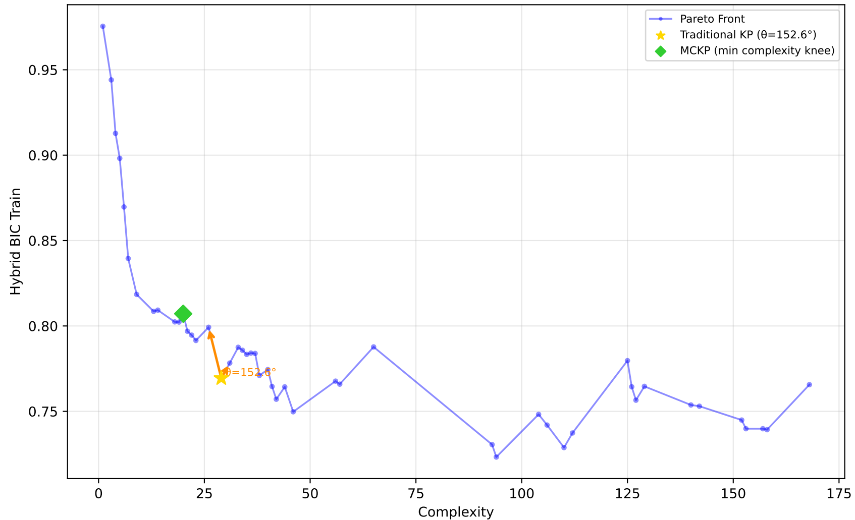
1096_FacultySalaries - Run 13 - MVP - Hybrid BIC Train \lambda_1=0.10 , \lambda_2=0.00 , \lambda_3=0.00 | Difficulty: 1.00 | Method: hmr
