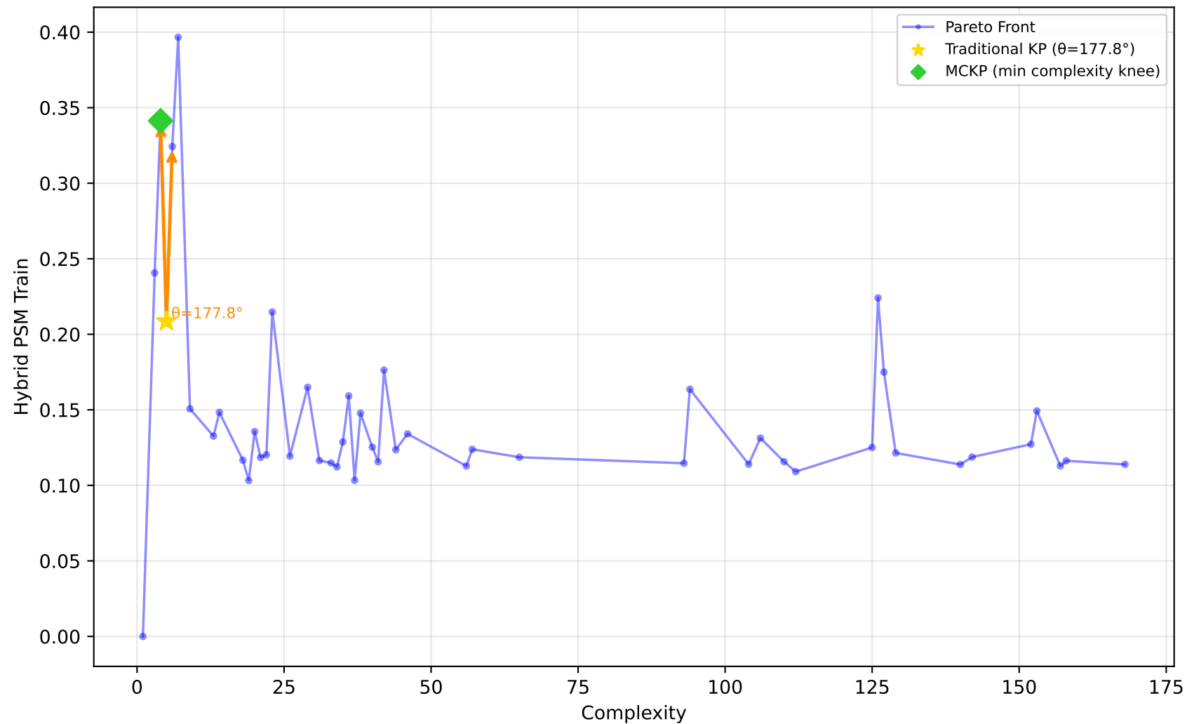
1096_FacultySalaries - Run 13 - MVP - Hybrid PSM Train \lambda_1=1.00, \lambda_2=0.00, \lambda_3=0.00 | Difficulty: 1.00 | Method: hmr
