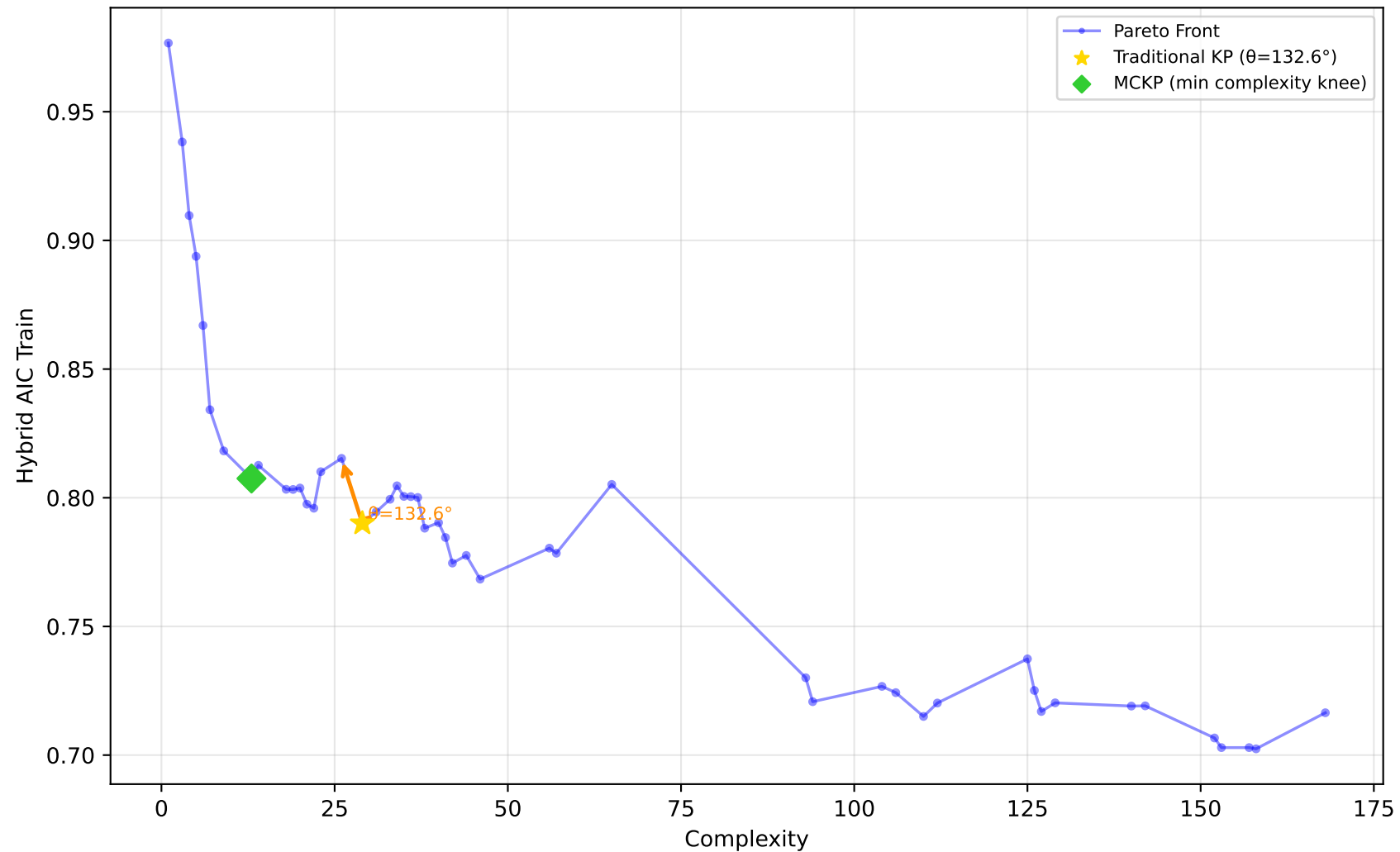
1096_FacultySalaries - Run 13 - SVP - Hybrid AIC Train \lambda_1=0.00 , \lambda_2=0.90 , \lambda_3=0.00 | Difficulty: 1.00 | Method: hmr
