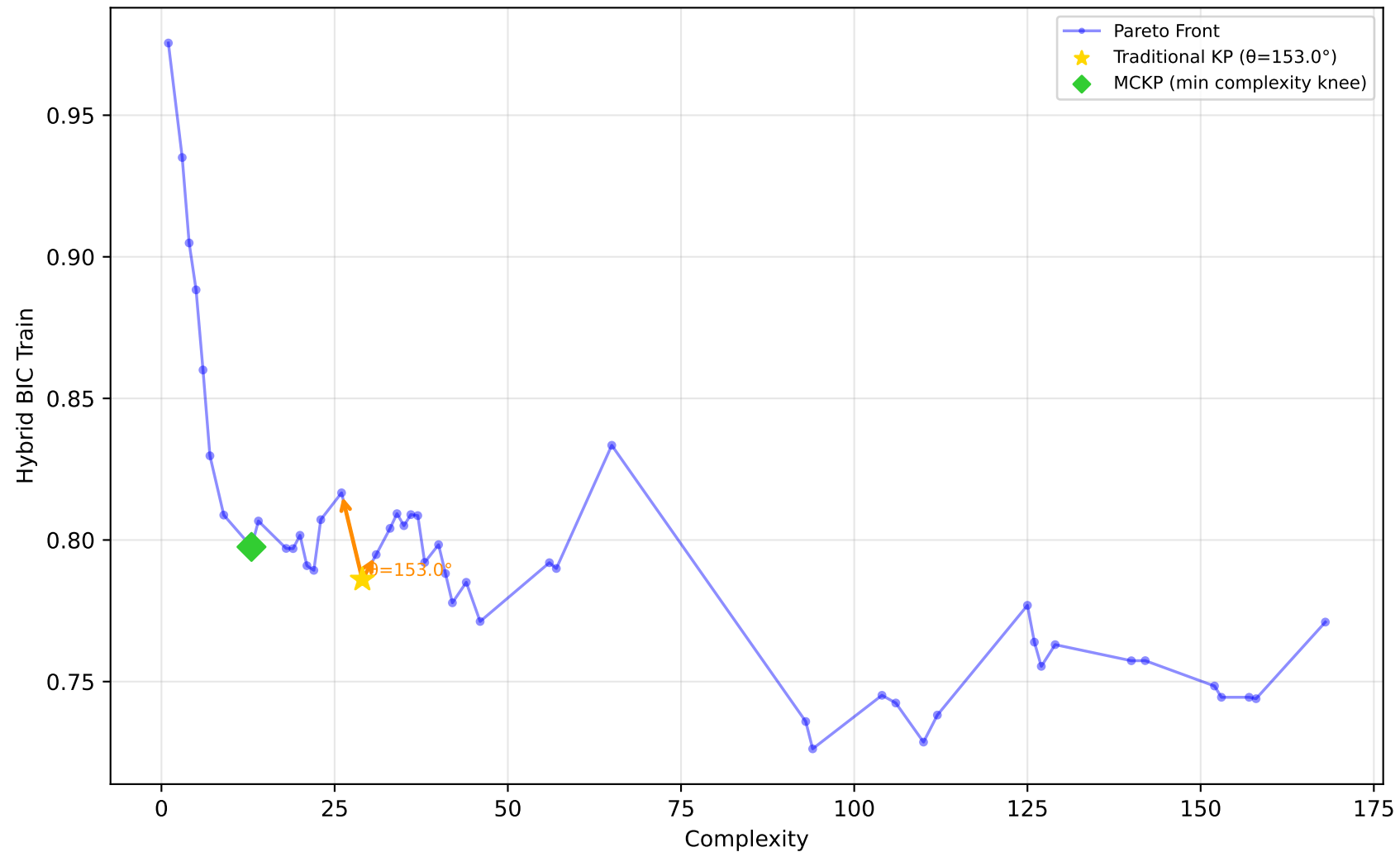
1096_FacultySalaries - Run 13 - SVP - Hybrid BIC Train \lambda_1=0.00 , \lambda_2=0.90 , \lambda_3=0.00 | Difficulty: 1.00 | Method: hmr
