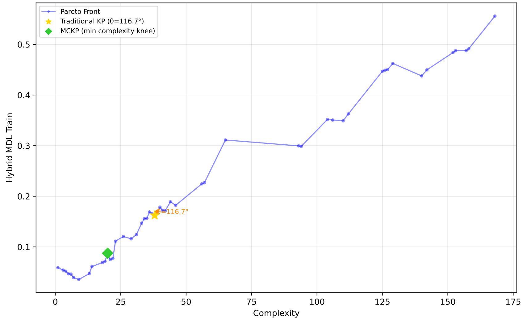
1096_FacultySalaries - Run 13 - SVP - Hybrid MDL Train \lambda_1=0.00 , \lambda_2=0.90 , \lambda_3=0.00 | Difficulty: 1.00 | Method: hmr
