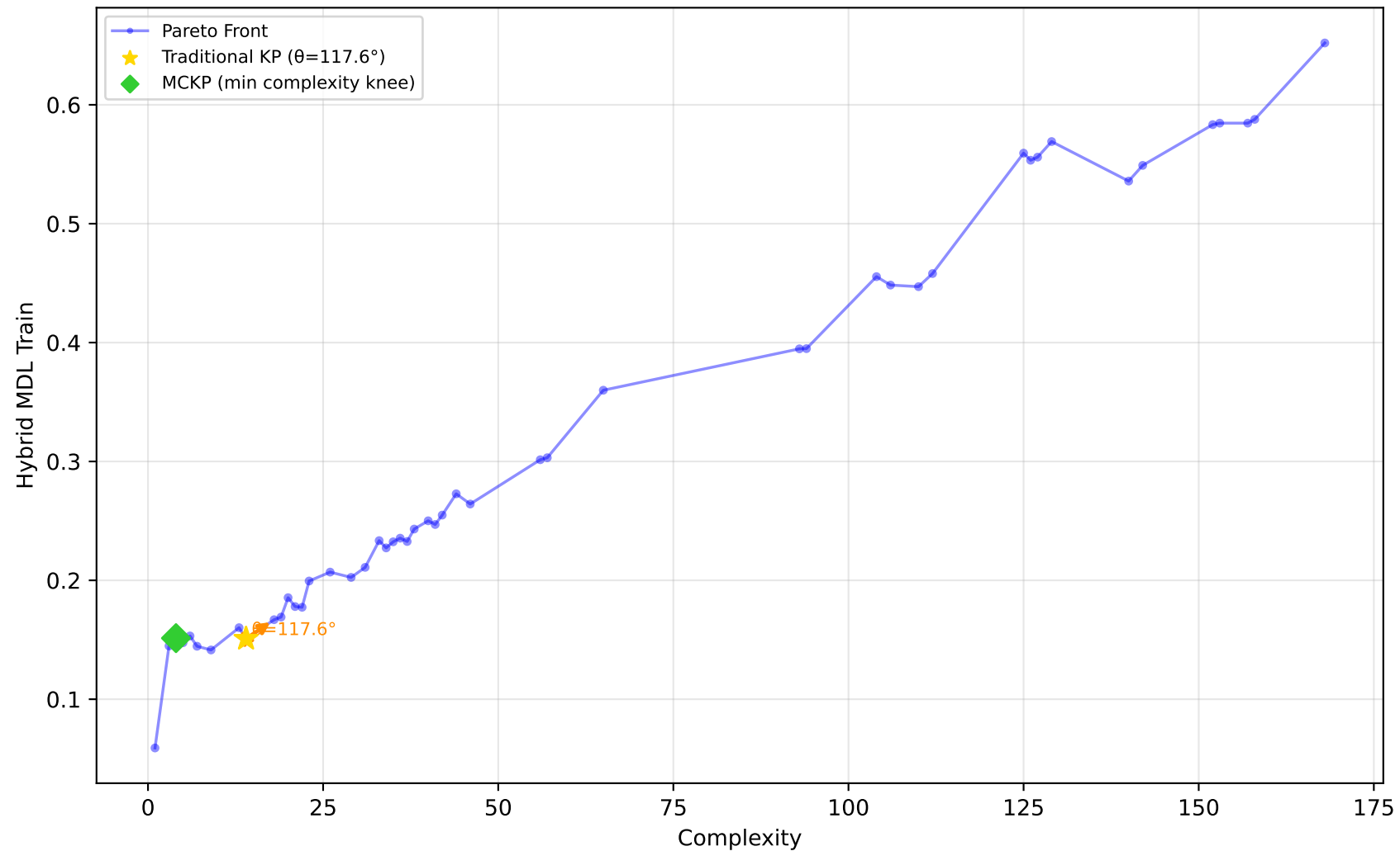
1096_FacultySalaries - Run 13 - SVP - Hybrid MDL Train \lambda_1=1.00, \lambda_2=0.00, \lambda_3=0.00 | Difficulty: 1.00 | Method: hmr
