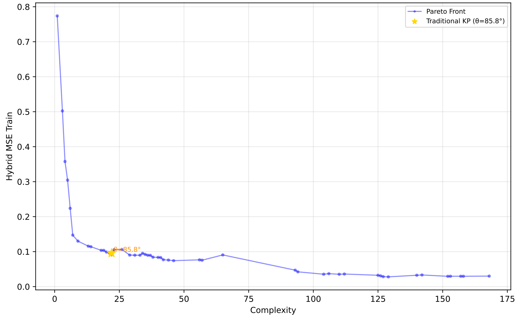
1096_FacultySalaries - Run 13 - SVP - Hybrid MSE Train \lambda_1=0.00 , \lambda_2=0.90 , \lambda_3=0.00 | Difficulty: 1.00 | Method: hmr
