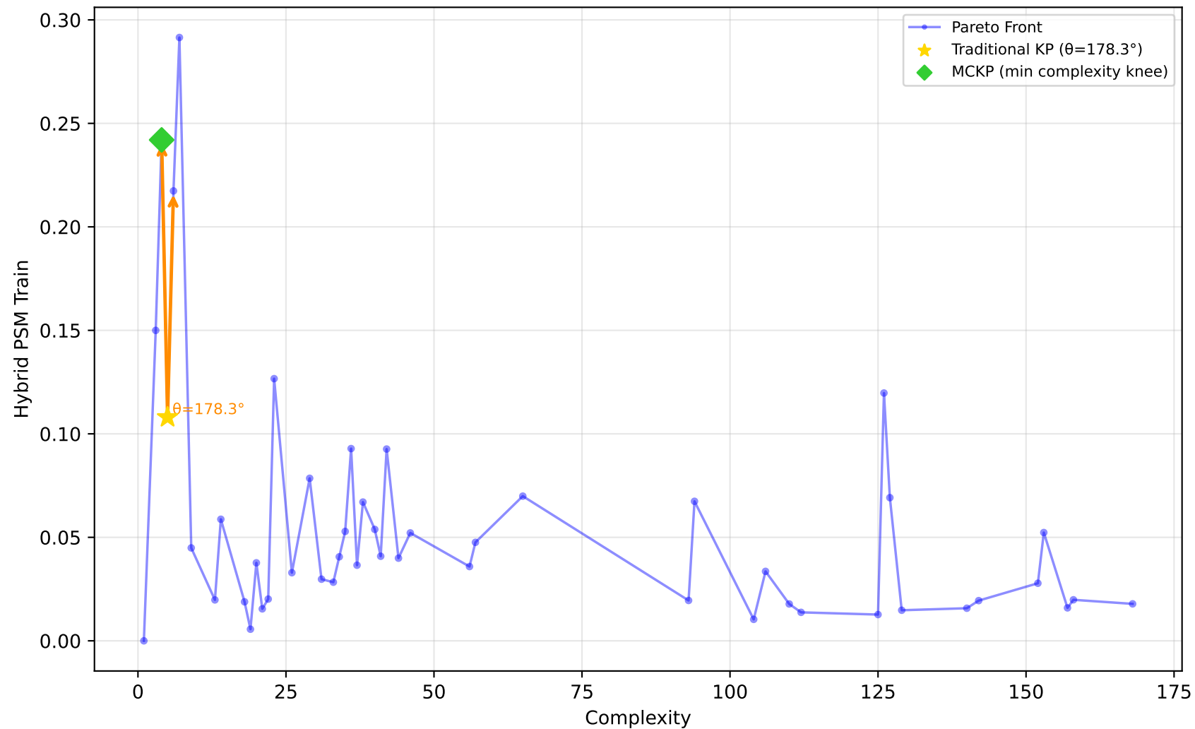
1096_FacultySalaries - Run 13 - SVP - Hybrid PSM Train \lambda_1=0.00 , \lambda_2=0.90 , \lambda_3=0.00 | Difficulty: 1.00 | Method: hmr
