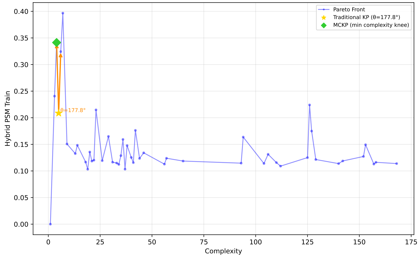
1096_FacultySalaries - Run 13 - SVP - Hybrid PSM Train \lambda_1=1.00 , \lambda_2=0.00 , \lambda_3=0.00 | Difficulty: 1.00 | Method: hmr
