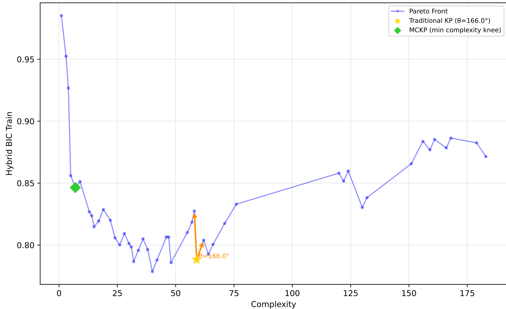
1096_FacultySalaries - Run 14 - MVP - Hybrid BIC Train \lambda_1=0.10 , \lambda_2=0.00 , \lambda_3=0.00 | Difficulty: 1.00 | Method: hmr
