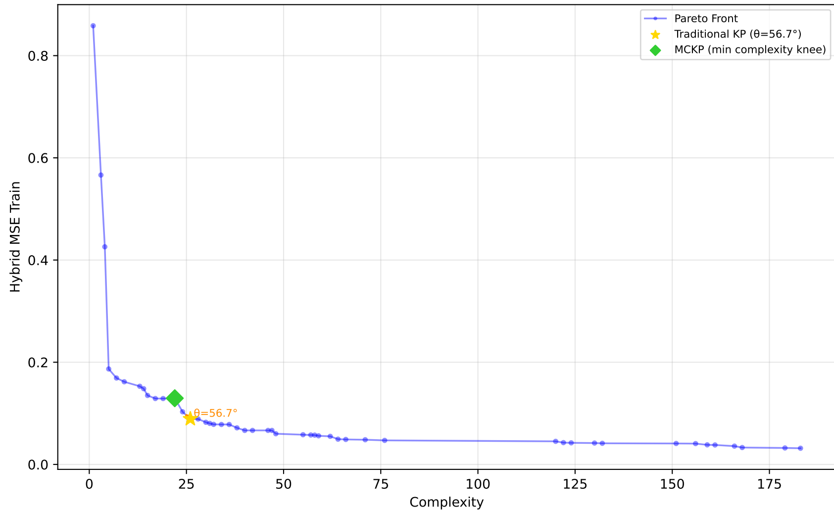
1096_FacultySalaries - Run 14 - MVP - Hybrid MSE Train \lambda_1=0.10 , \lambda_2=0.00 , \lambda_3=0.00 | Difficulty: 1.00 | Method: hmr
