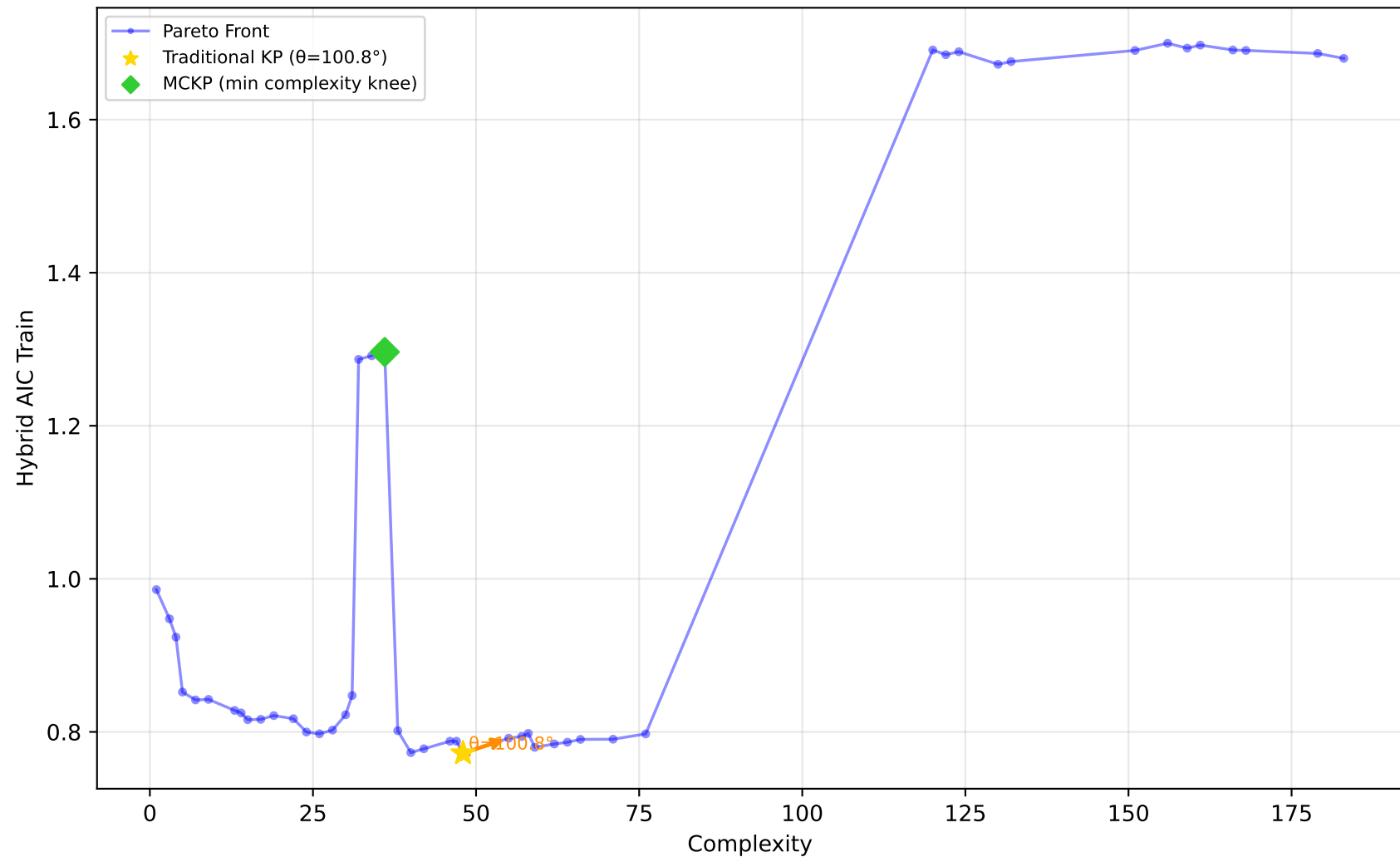
1096_FacultySalaries - Run 14 - SVP - Hybrid AIC Train \lambda_1=0.00 , \lambda_2=0.90 , \lambda_3=0.00 | Difficulty: 1.00 | Method: hmr
