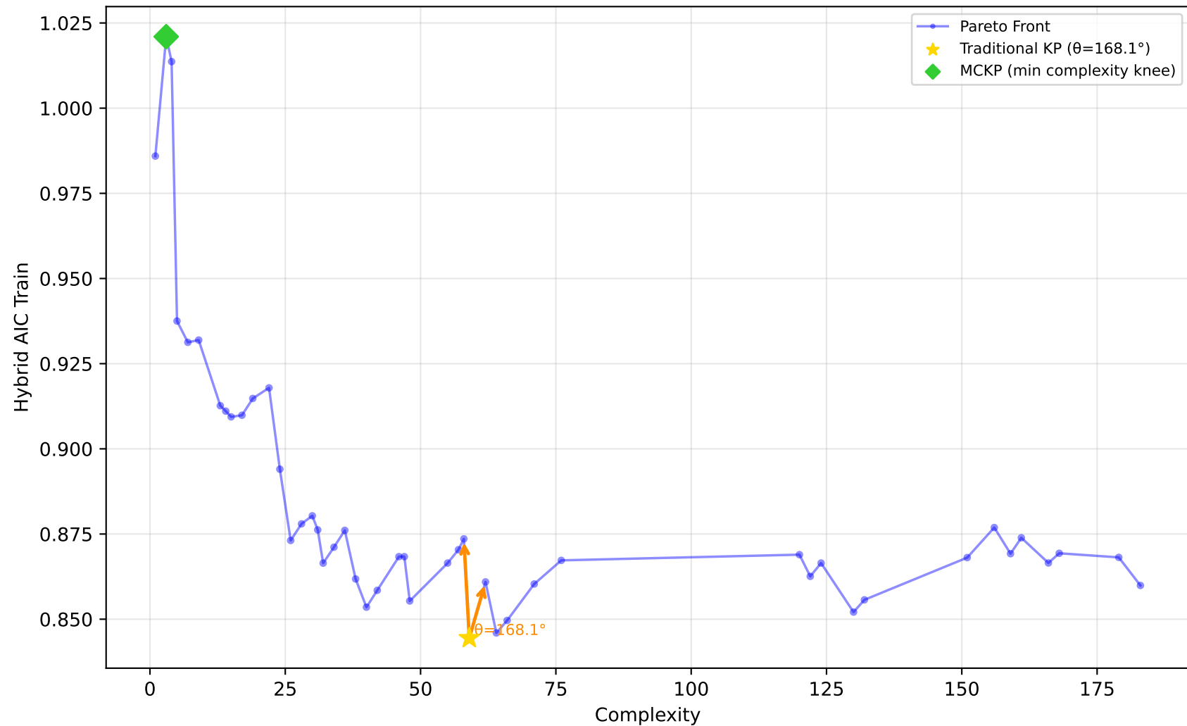
1096_FacultySalaries - Run 14 - SVP - Hybrid AIC Train \lambda_1=1.00 , \lambda_2=0.00 , \lambda_3=0.00 | Difficulty: 1.00 | Method: hmr
