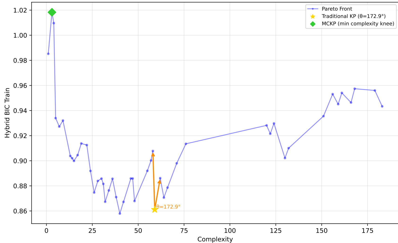
1096_FacultySalaries - Run 14 - SVP - Hybrid BIC Train \lambda_1=1.00 , \lambda_2=0.00 , \lambda_3=0.00 | Difficulty: 1.00 | Method: hmr
