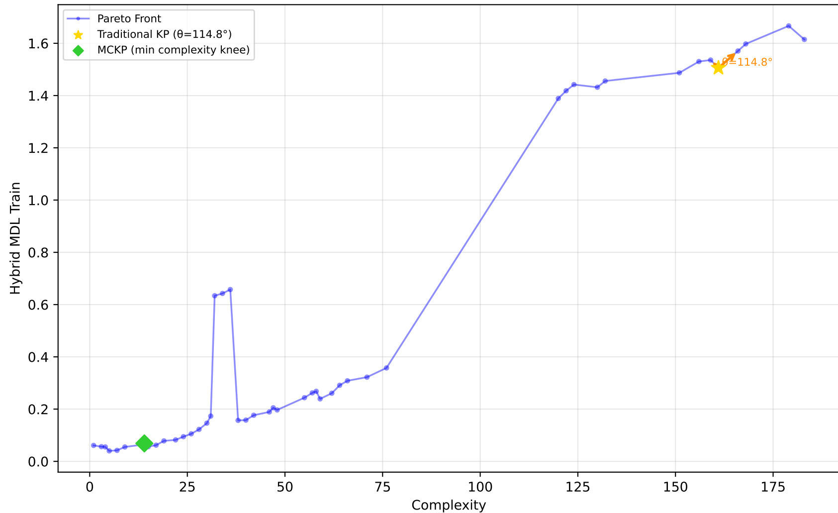
1096_FacultySalaries - Run 14 - SVP - Hybrid MDL Train \lambda_1=0.00, \lambda_2=0.90, \lambda_3=0.00 | Difficulty: 1.00 | Method: hmr
