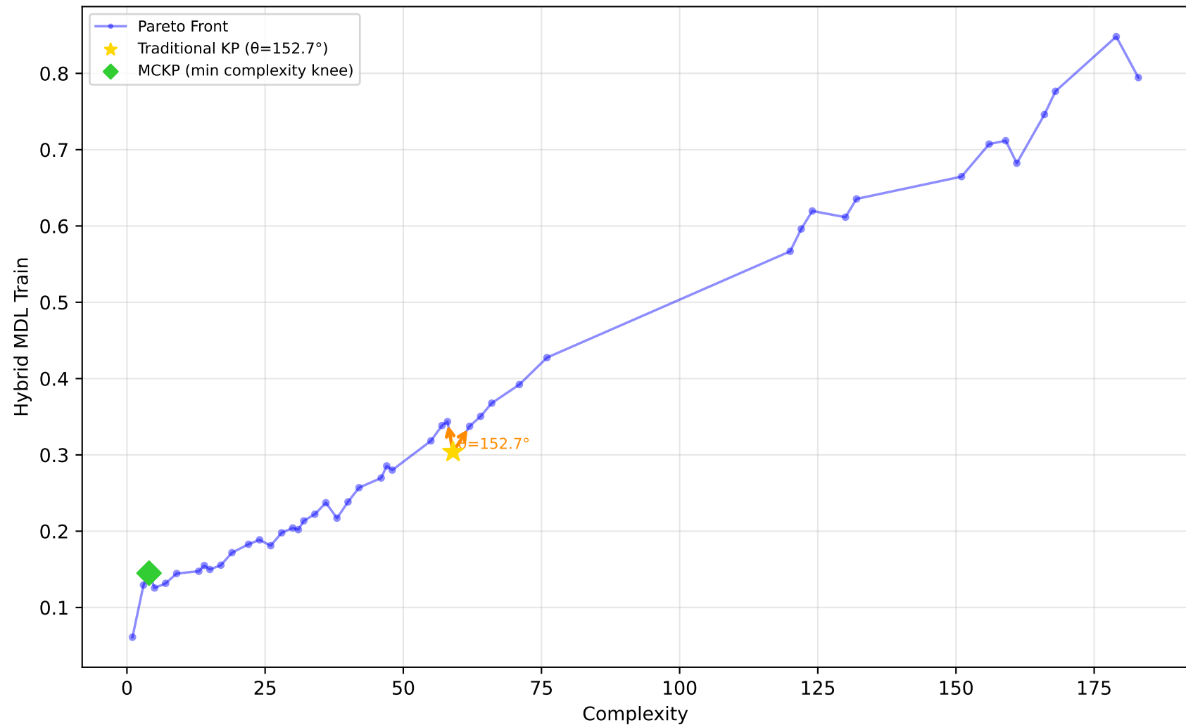
\lambda_1=1.00, \lambda_2=0.00, \lambda_3=0.00 | Difficulty: 1.00 | Method: hmr
