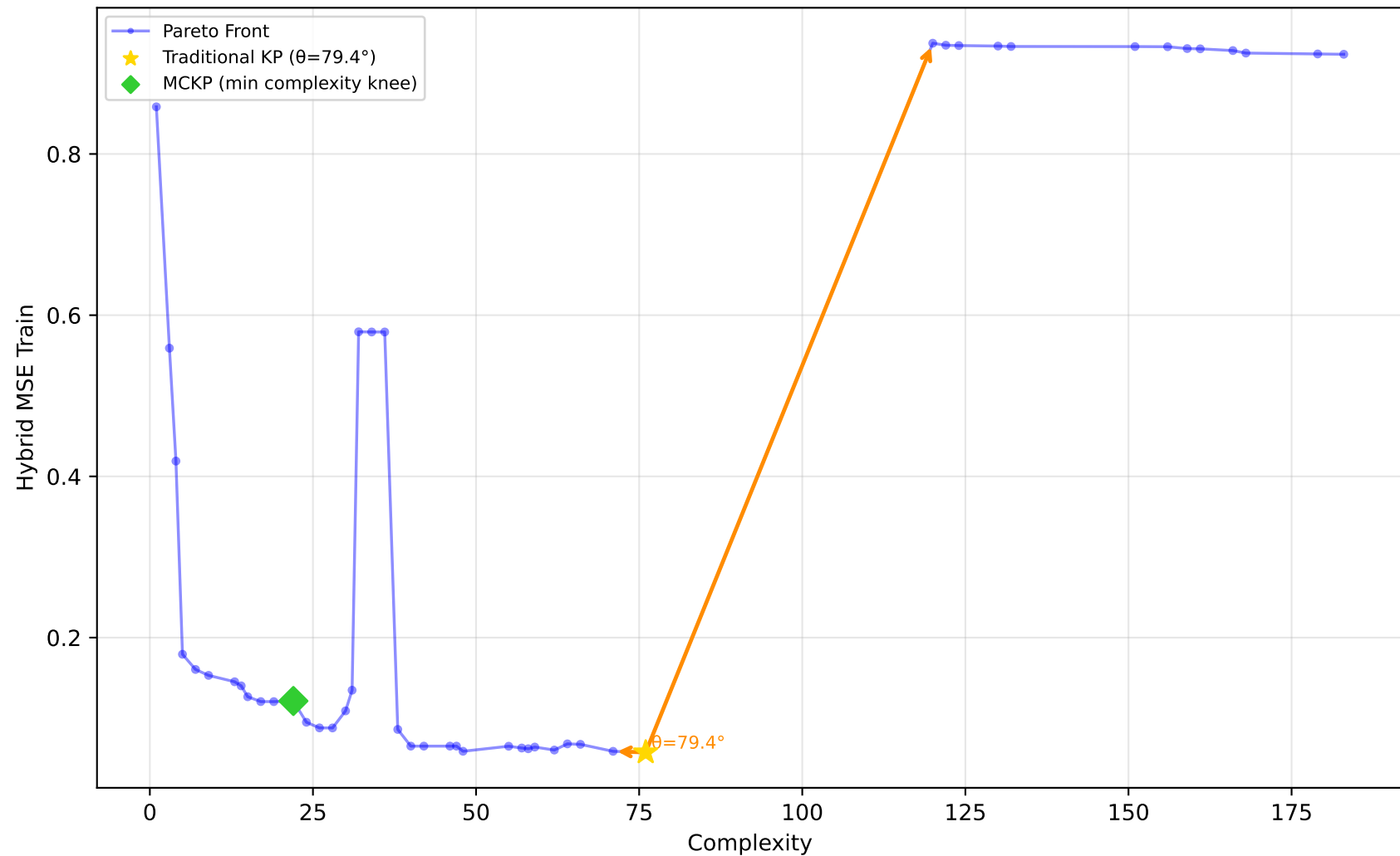
1096_FacultySalaries - Run 14 - SVP - Hybrid MSE Train \lambda_1=0.00, \lambda_2=0.90, \lambda_3=0.00 | Difficulty: 1.00 | Method: hmr
