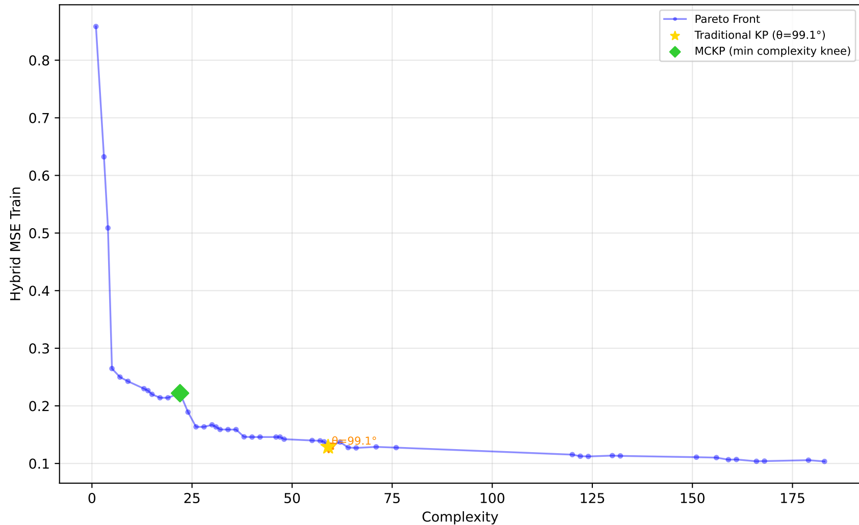
1096_FacultySalaries - Run 14 - SVP - Hybrid MSE Train \lambda_1=1.00, \lambda_2=0.00, \lambda_3=0.00 | Difficulty: 1.00 | Method: hmr
