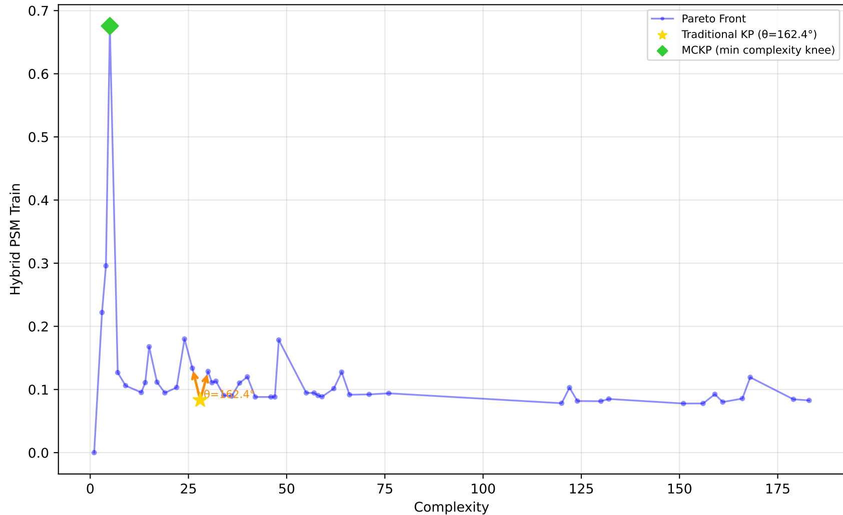
1096_FacultySalaries - Run 14 - SVP - Hybrid PSM Train \lambda_1=1.00 , \lambda_2=0.00 , \lambda_3=0.00 | Difficulty: 1.00 | Method: hmr
