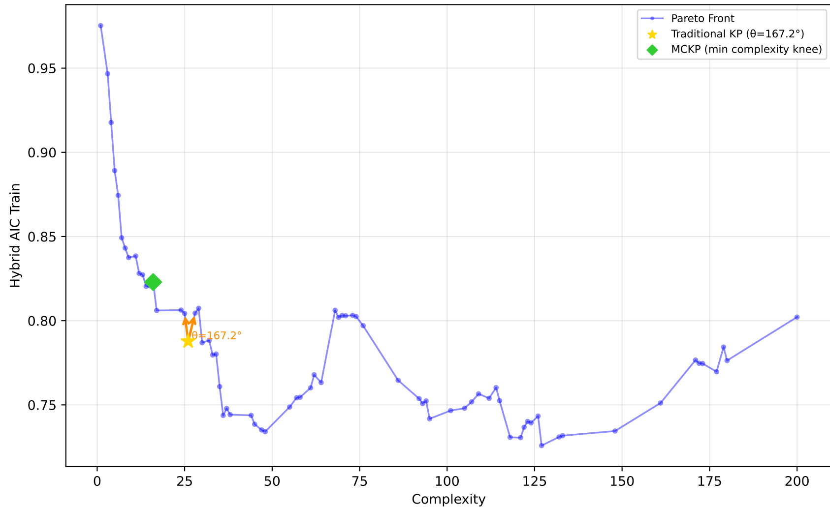
1096_FacultySalaries - Run 15 - MVP - Hybrid AIC Train \lambda_1=0.10, \lambda_2=0.00, \lambda_3=0.00 | Difficulty: 0.51 | Method: mckp
