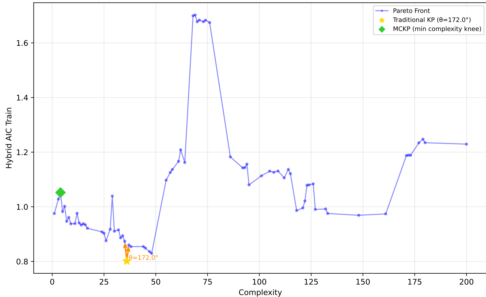
1096_FacultySalaries - Run 15 - MVP - Hybrid AIC Train \lambda_1=1.00 , \lambda_2=0.00 , \lambda_3=0.00 | Difficulty: 0.51 | Method: mckp
