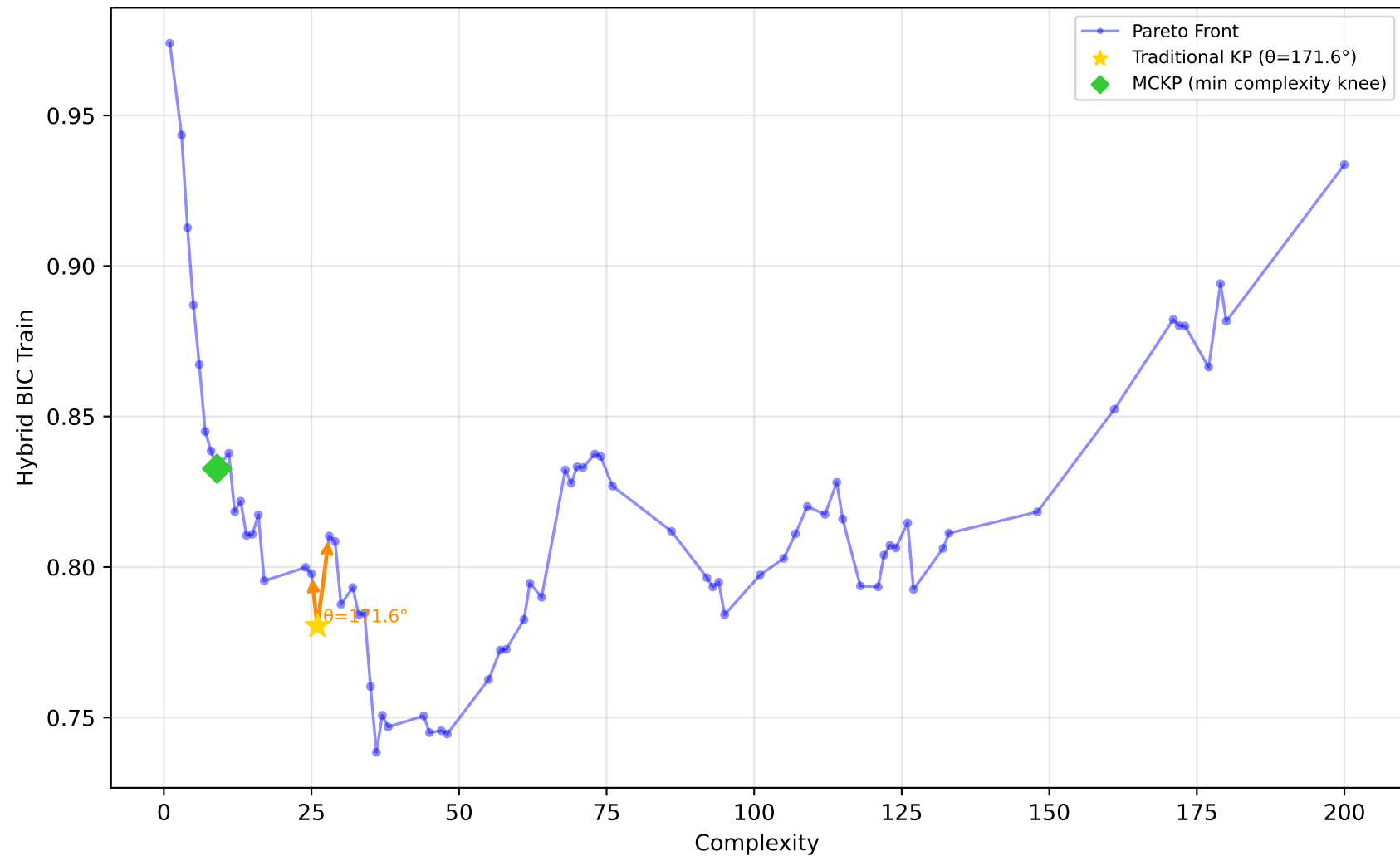
1096_FacultySalaries - Run 15 - MVP - Hybrid BIC Train \lambda_1=0.10, \lambda_2=0.00, \lambda_3=0.00 | Difficulty: 0.51 | Method: mckp
