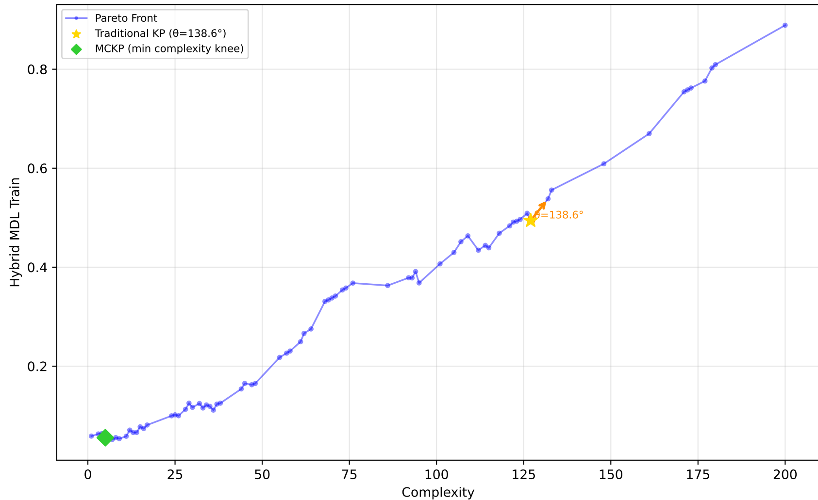
1096_FacultySalaries - Run 15 - MVP - Hybrid MDL Train \lambda_1=0.10, \lambda_2=0.00, \lambda_3=0.00 | Difficulty: 0.51 | Method: mckp
