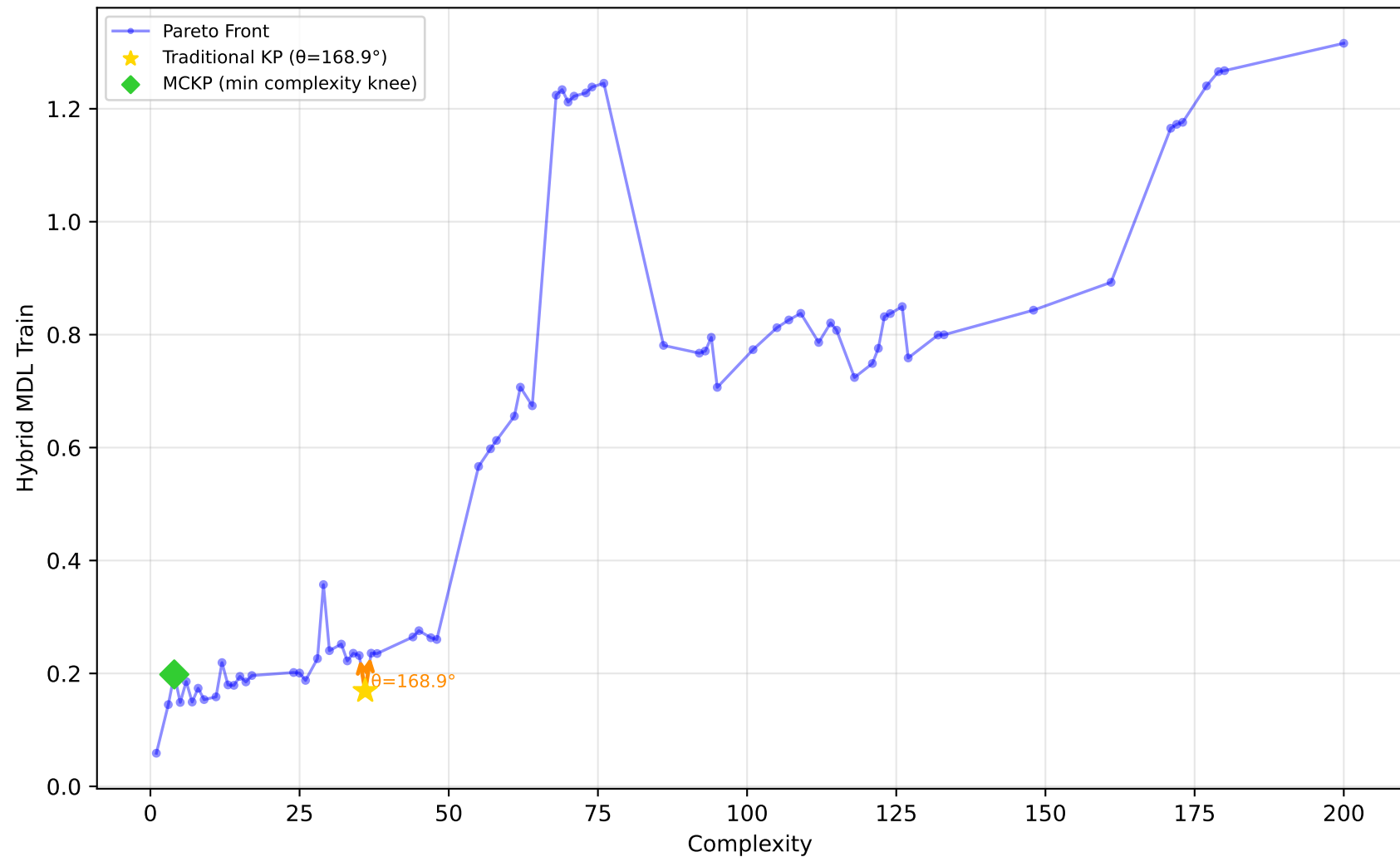
1096_FacultySalaries - Run 15 - MVP - Hybrid MDL Train \lambda_1=1.00 , \lambda_2=0.00 , \lambda_3=0.00 | Difficulty: 0.51 | Method: mckp
