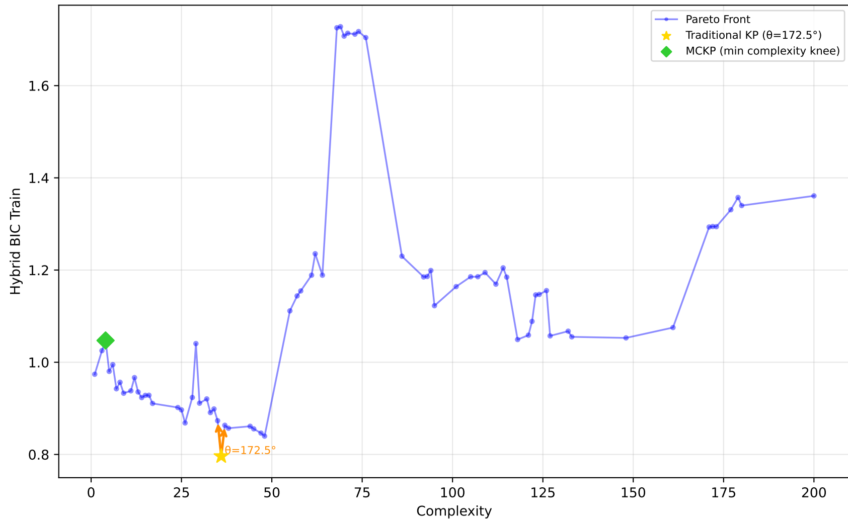
1096_FacultySalaries - Run 15 - SVP - Hybrid BIC Train \lambda_1=1.00, \lambda_2=0.00, \lambda_3=0.00 | Difficulty: 0.51 | Method: mckp
