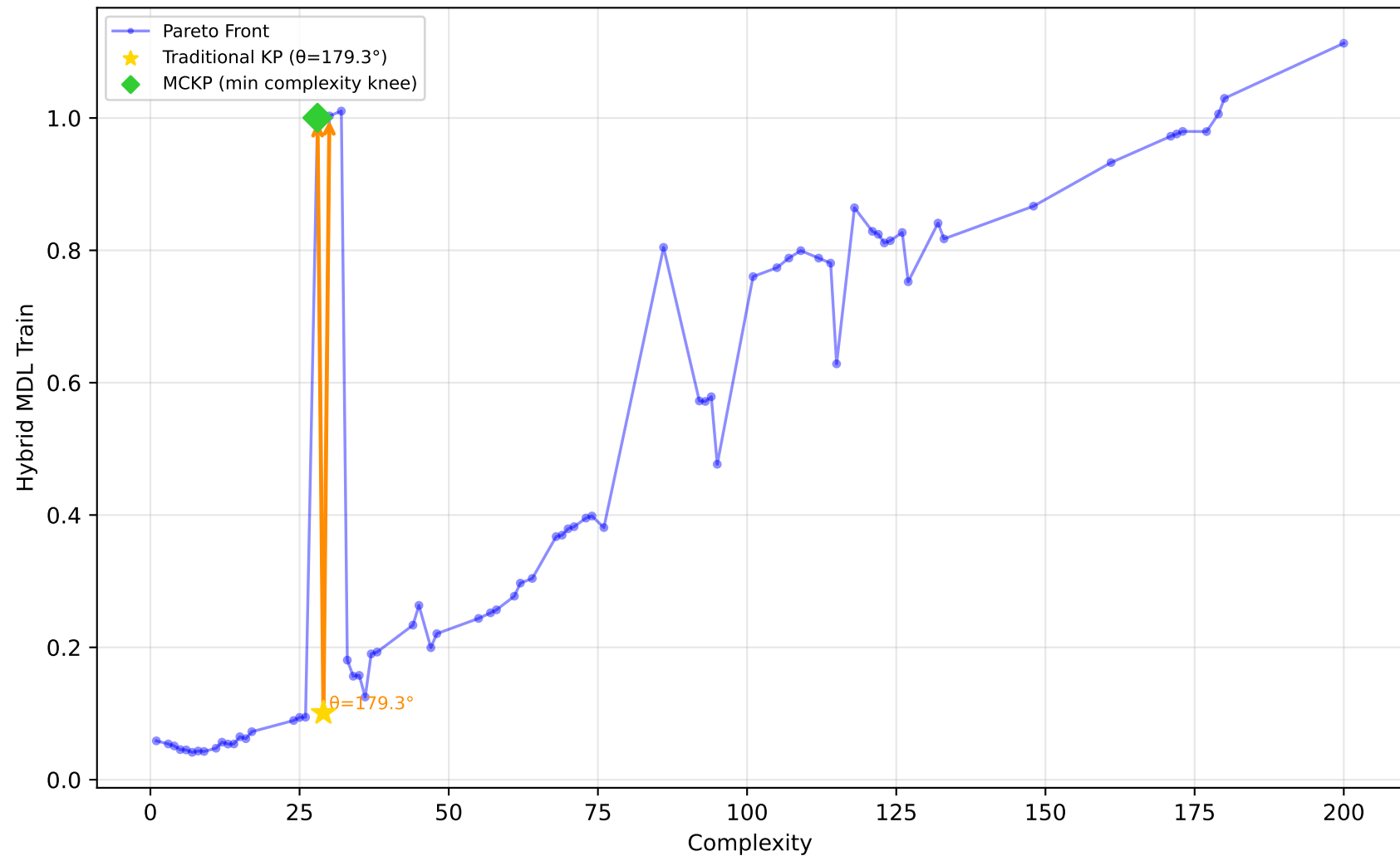
1096_FacultySalaries - Run 15 - SVP - Hybrid MDL Train \lambda_1=0.00, \lambda_2=0.90, \lambda_3=0.00 | Difficulty: 0.51 | Method: mckp
