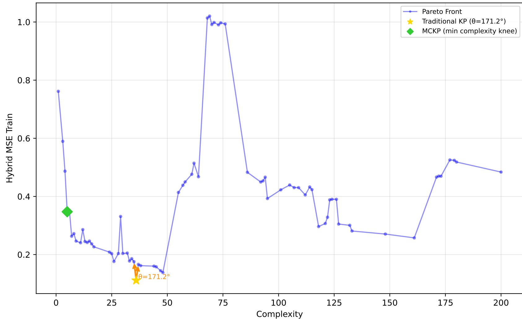
1096_FacultySalaries - Run 15 - SVP - Hybrid MSE Train \lambda_1=1.00, \lambda_2=0.00, \lambda_3=0.00 | Difficulty: 0.51 | Method: mckp
