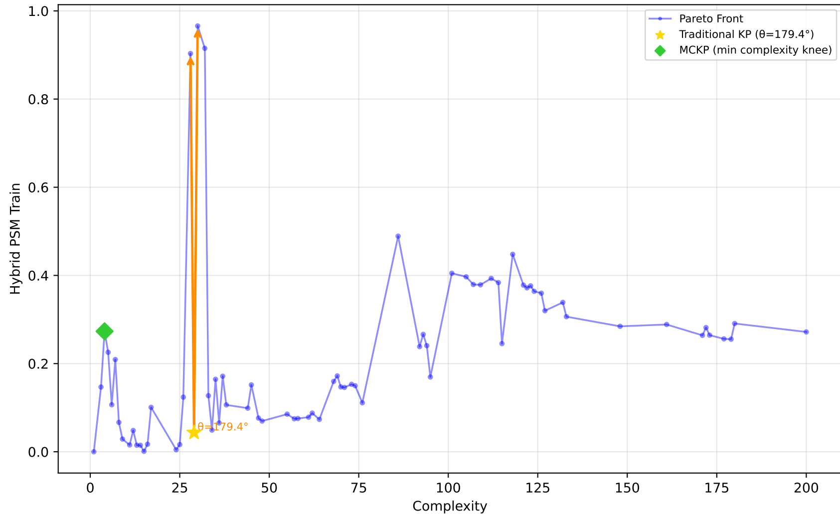
1096_FacultySalaries - Run 15 - SVP - Hybrid PSM Train \lambda_1=0.00, \lambda_2=0.90, \lambda_3=0.00 | Difficulty: 0.51 | Method: mckp
