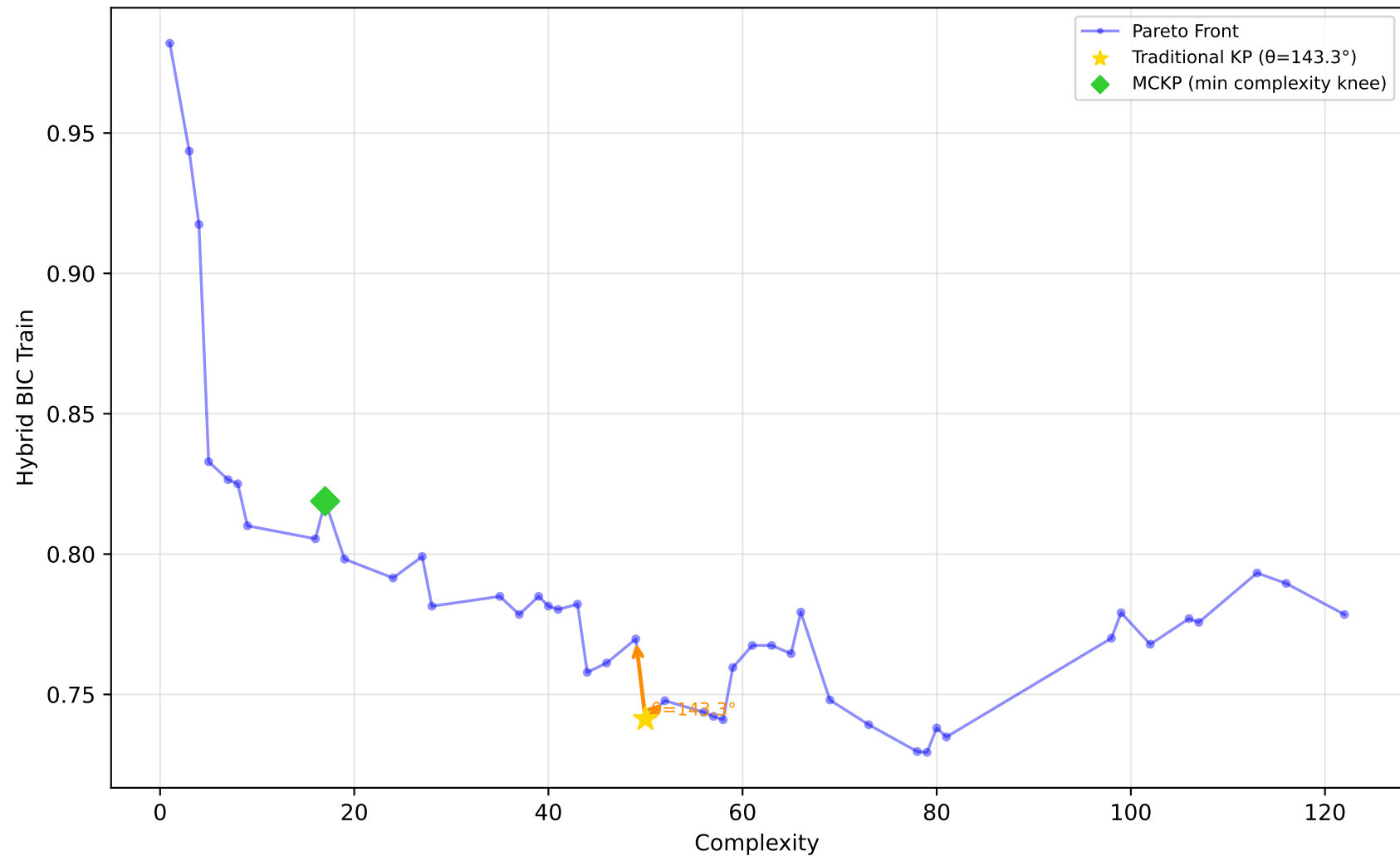
1096_FacultySalaries - Run 16 - MVP - Hybrid BIC Train \lambda_1=0.10 , \lambda_2=0.00 , \lambda_3=0.00 | Difficulty: 0.80 | Method: hmr
