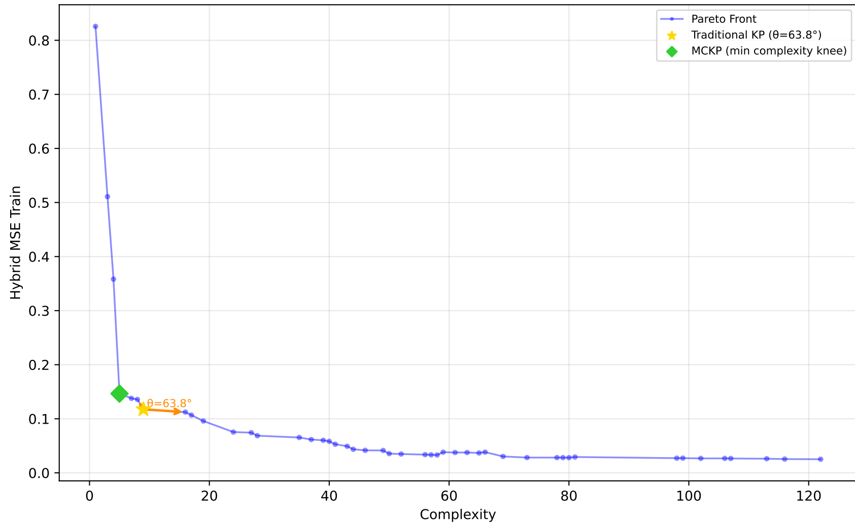
1096_FacultySalaries - Run 16 - MVP - Hybrid MSE Train \lambda_1=0.10, \lambda_2=0.00, \lambda_3=0.00 | Difficulty: 0.80 | Method: hmr
