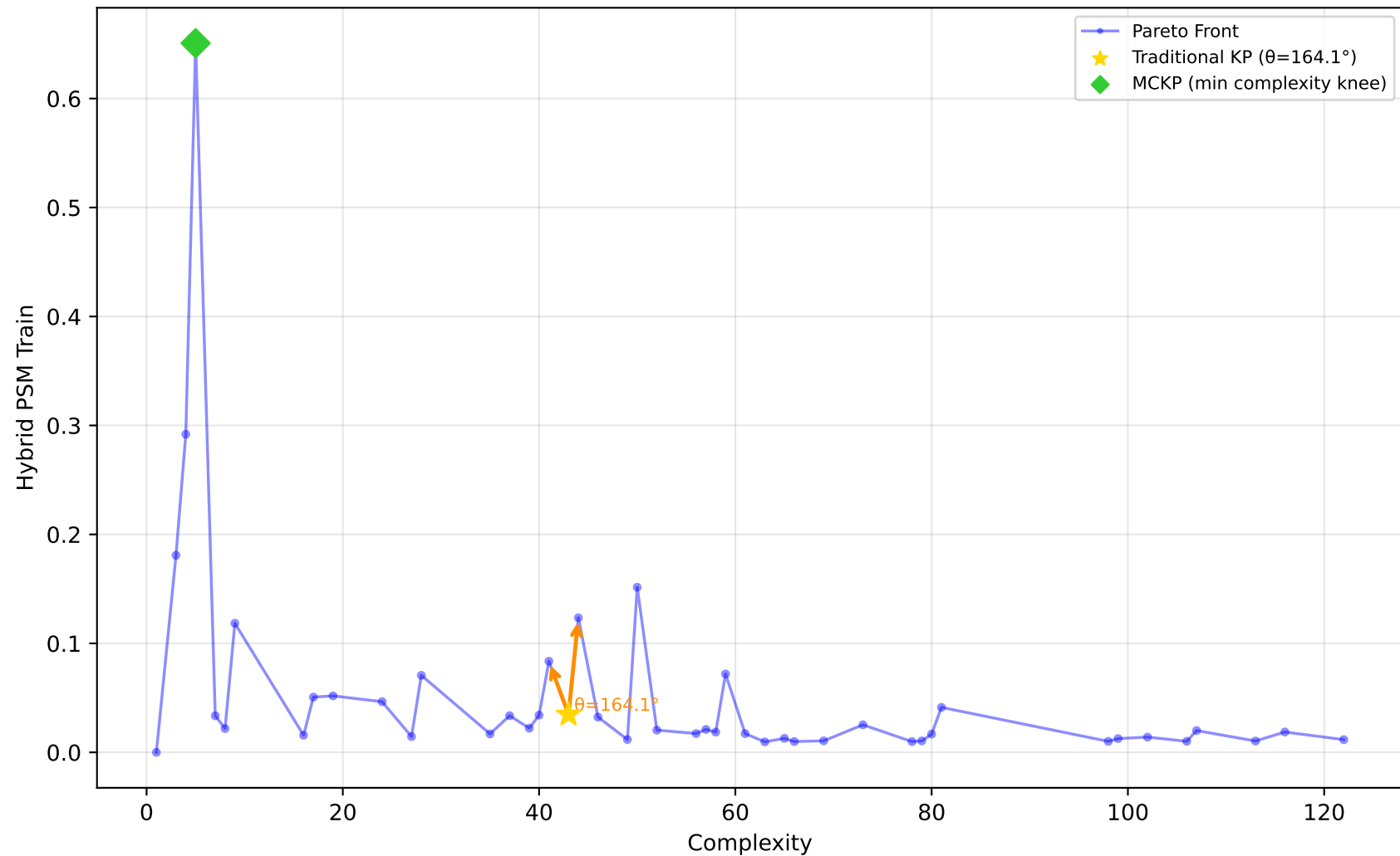
1096_FacultySalaries - Run 16 - MVP - Hybrid PSM Train \lambda_1=0.10 , \lambda_2=0.00 , \lambda_3=0.00 | Difficulty: 0.80 | Method: hmr
