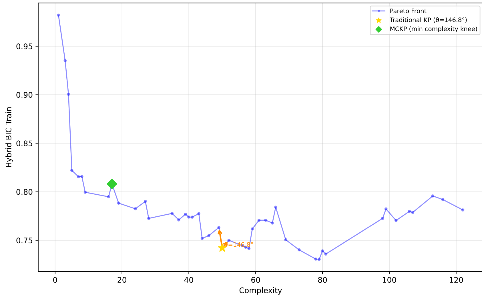
1096_FacultySalaries - Run 16 - SVP - Hybrid BIC Train \lambda_1=0.00 , \lambda_2=0.90 , \lambda_3=0.00 | Difficulty: 0.80 | Method: hmr
