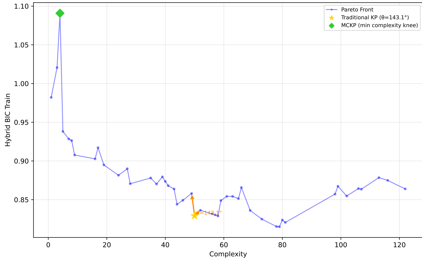
1096_FacultySalaries - Run 16 - SVP - Hybrid BIC Train \lambda_1=1.00 , \lambda_2=0.00 , \lambda_3=0.00 | Difficulty: 0.80 | Method: hmr
