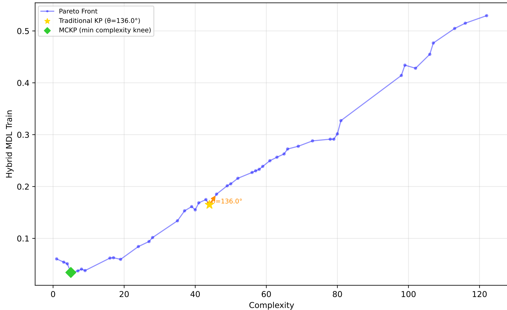
1096_FacultySalaries - Run 16 - SVP - Hybrid MDL Train \lambda_1=0.00, \lambda_2=0.90, \lambda_3=0.00 | Difficulty: 0.80 | Method: hmr
