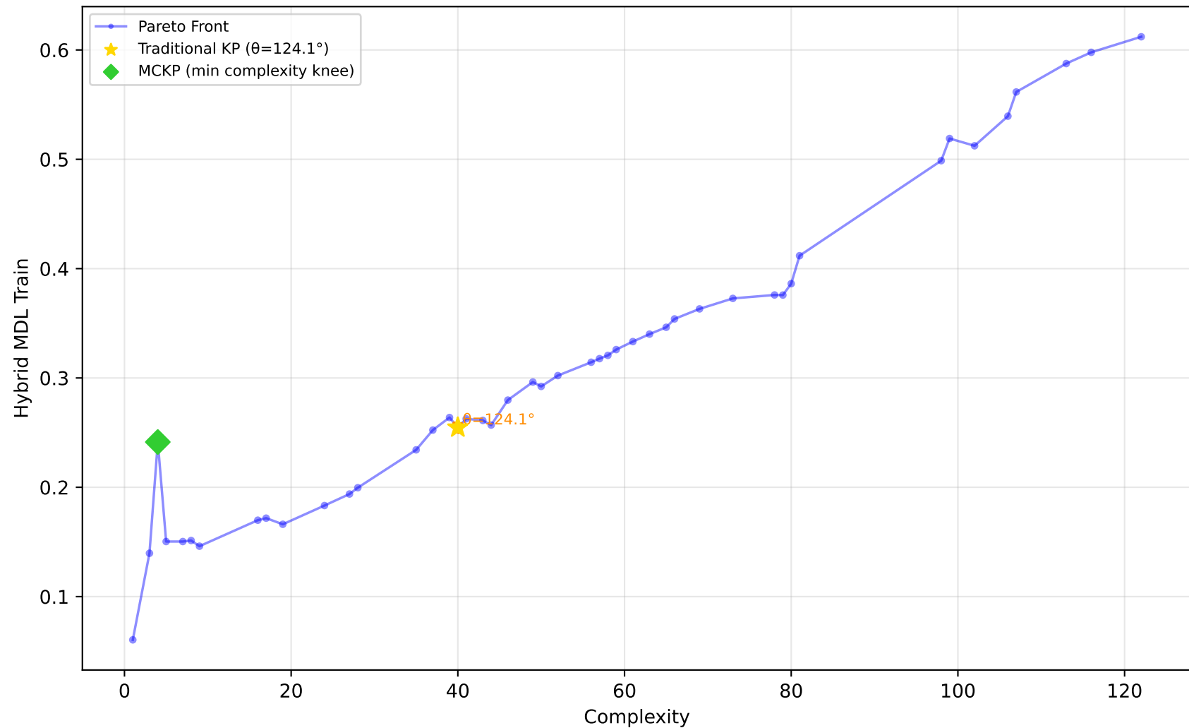
1096_FacultySalaries - Run 16 - SVP - Hybrid MDL Train \lambda_1=1.00 , \lambda_2=0.00 , \lambda_3=0.00 | Difficulty: 0.80 | Method: hmr
