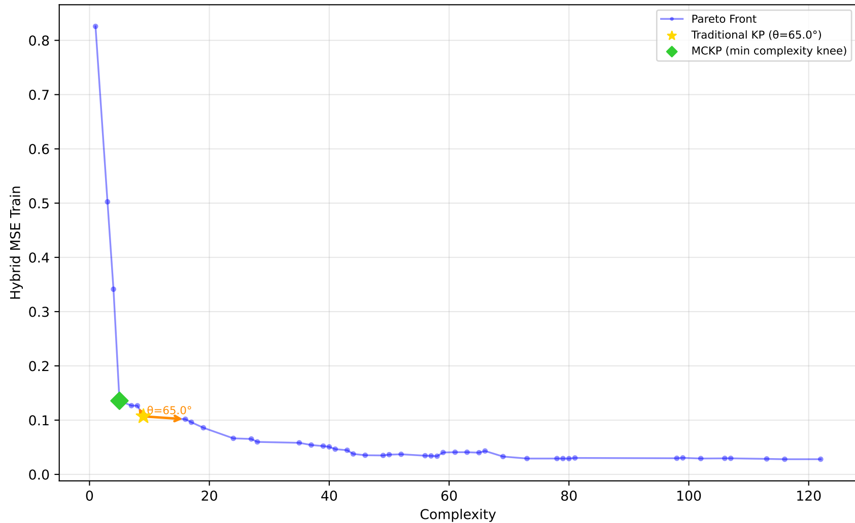
1096_FacultySalaries - Run 16 - SVP - Hybrid MSE Train \lambda_1=0.00 , \lambda_2=0.90 , \lambda_3=0.00 | Difficulty: 0.80 | Method: hmr
