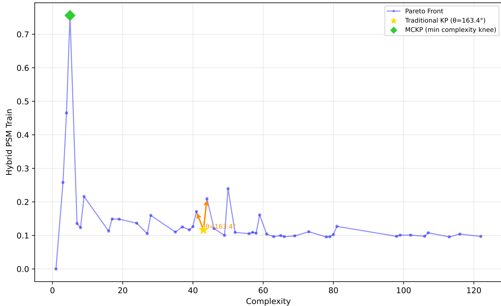
1096_FacultySalaries - Run 16 - SVP - Hybrid PSM Train \lambda_1=1.00 , \lambda_2=0.00 , \lambda_3=0.00 | Difficulty: 0.80 | Method: hmr
