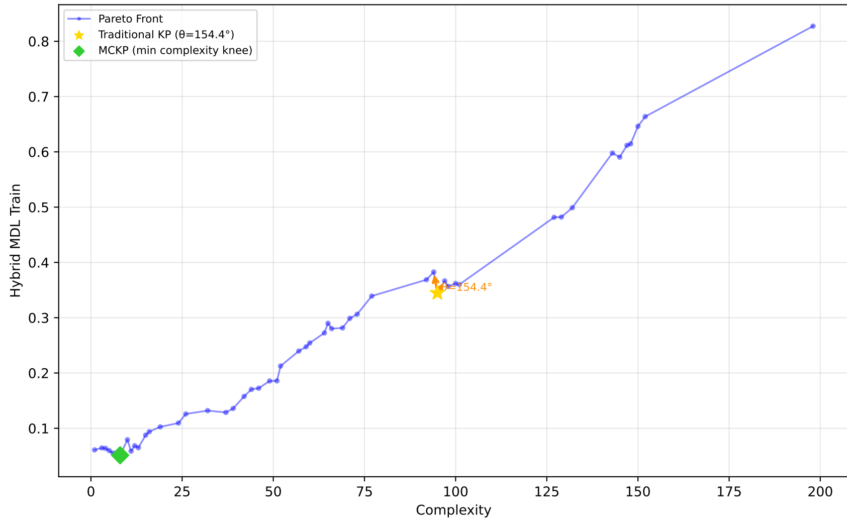
1096_FacultySalaries - Run 17 - MVP - Hybrid MDL Train \lambda_1=0.10, \lambda_2=0.00, \lambda_3=0.00 | Difficulty: 1.00 | Method: hmr
