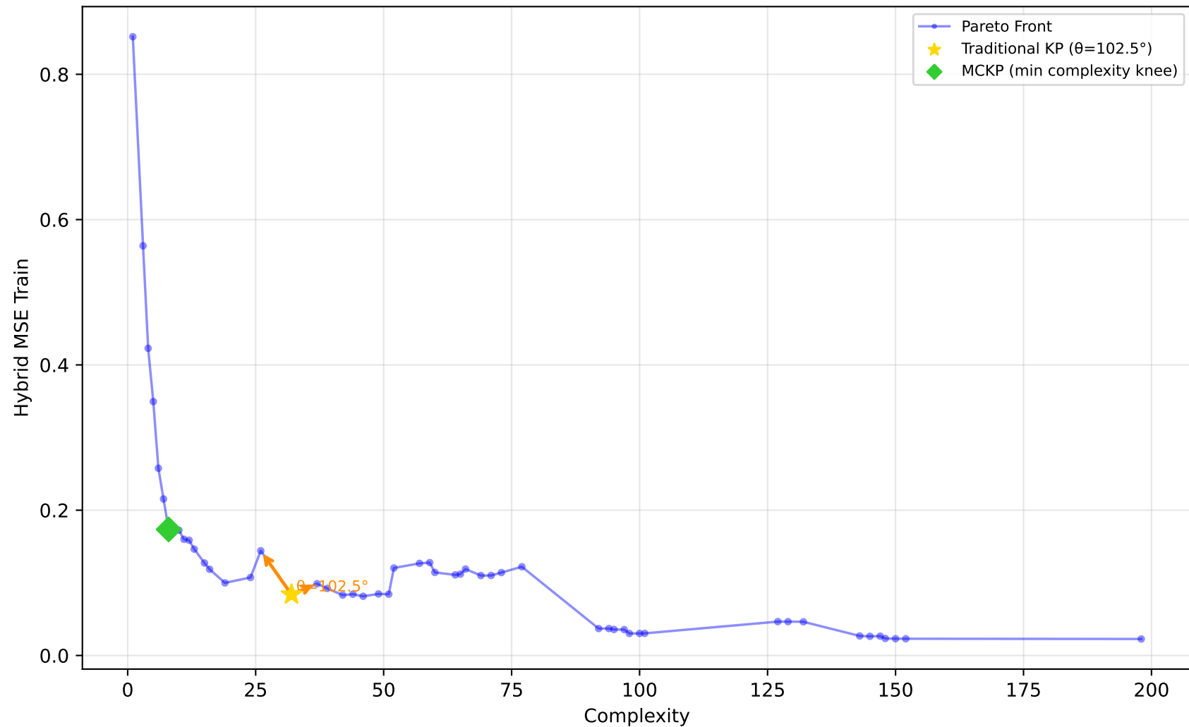
1096_FacultySalaries - Run 17 - MVP - Hybrid MSE Train \lambda_1=0.10, \lambda_2=0.00, \lambda_3=0.00 | Difficulty: 1.00 | Method: hmr
