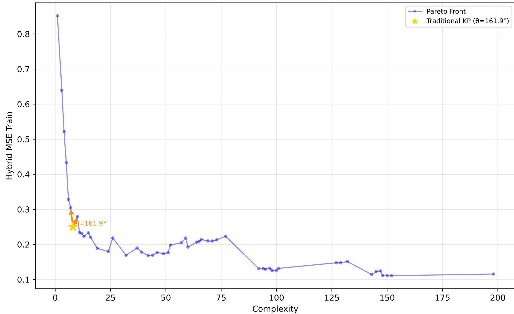
1096_FacultySalaries - Run 17 - MVP - Hybrid MSE Train \lambda_1=1.00, \lambda_2=0.00, \lambda_3=0.00 | Difficulty: 1.00 | Method: hmr
