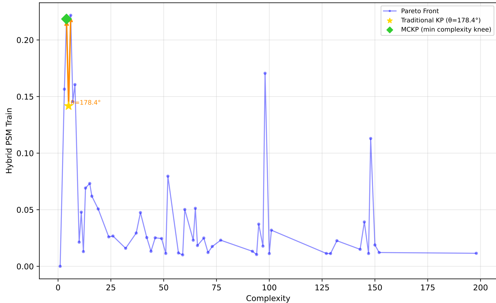
1096_FacultySalaries - Run 17 - MVP - Hybrid PSM Train \lambda_1=0.10 , \lambda_2=0.00 , \lambda_3=0.00 | Difficulty: 1.00 | Method: hmr
