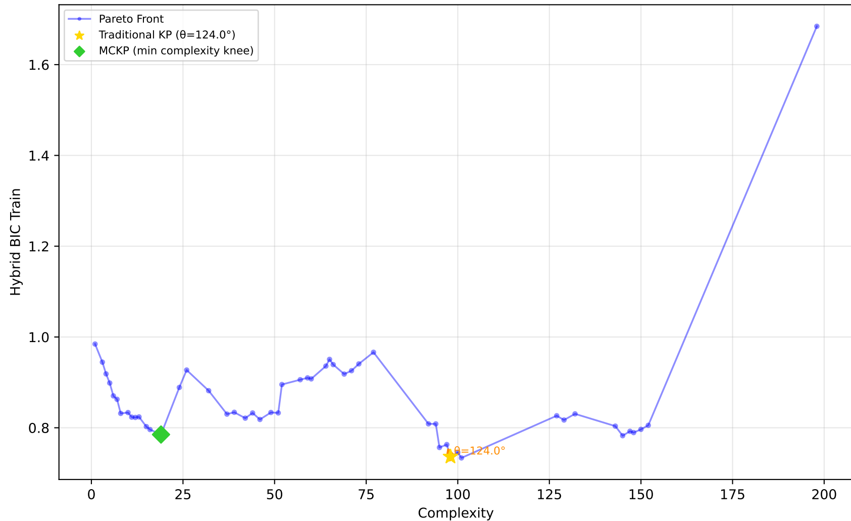
1096_FacultySalaries - Run 17 - SVP - Hybrid BIC Train \lambda_1=0.00, \lambda_2=0.90, \lambda_3=0.00 | Difficulty: 1.00 | Method: hmr
