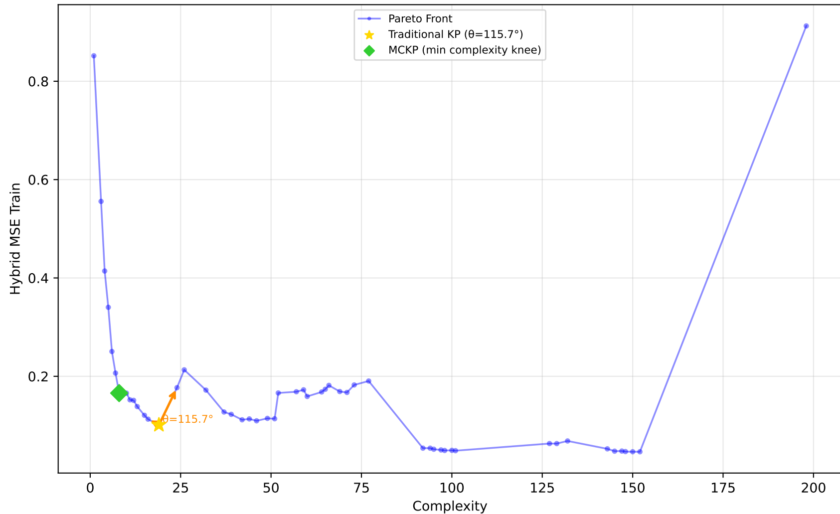
1096_FacultySalaries - Run 17 - SVP - Hybrid MSE Train \lambda_1=0.00, \lambda_2=0.90, \lambda_3=0.00 | Difficulty: 1.00 | Method: hmr
