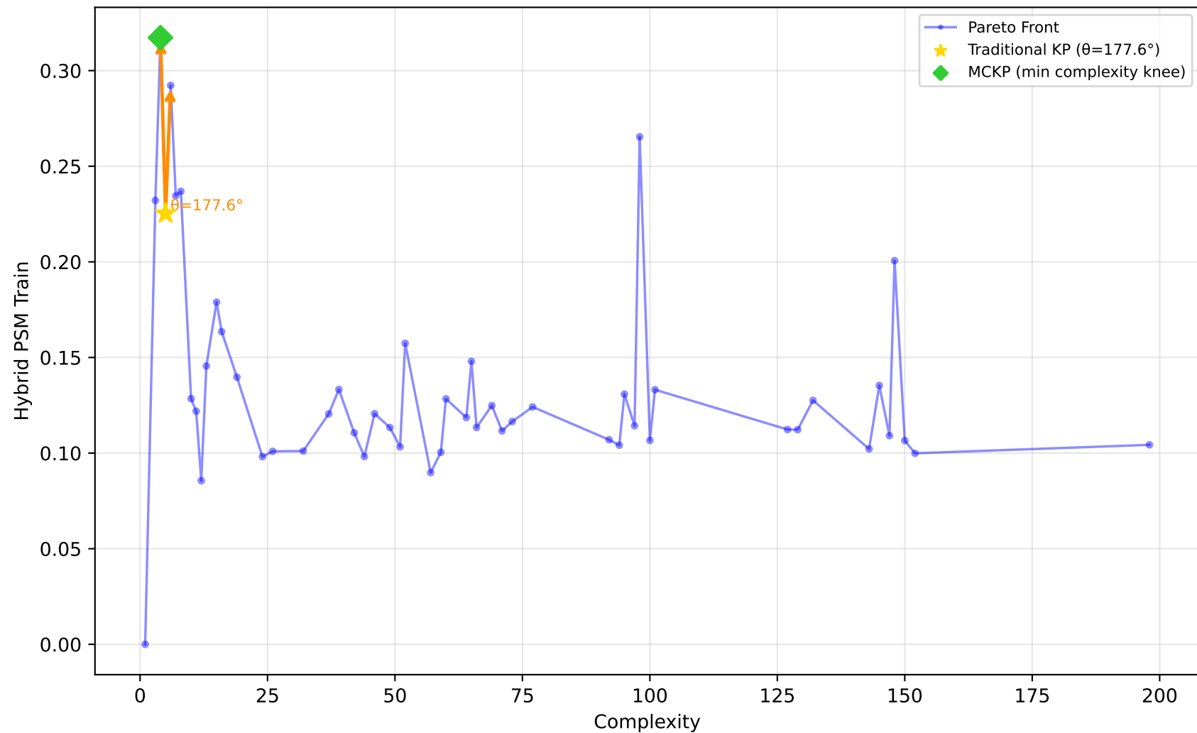
1096_FacultySalaries - Run 17 - SVP - Hybrid PSM Train \lambda_1=1.00, \lambda_2=0.00, \lambda_3=0.00 | Difficulty: 1.00 | Method: hmr
