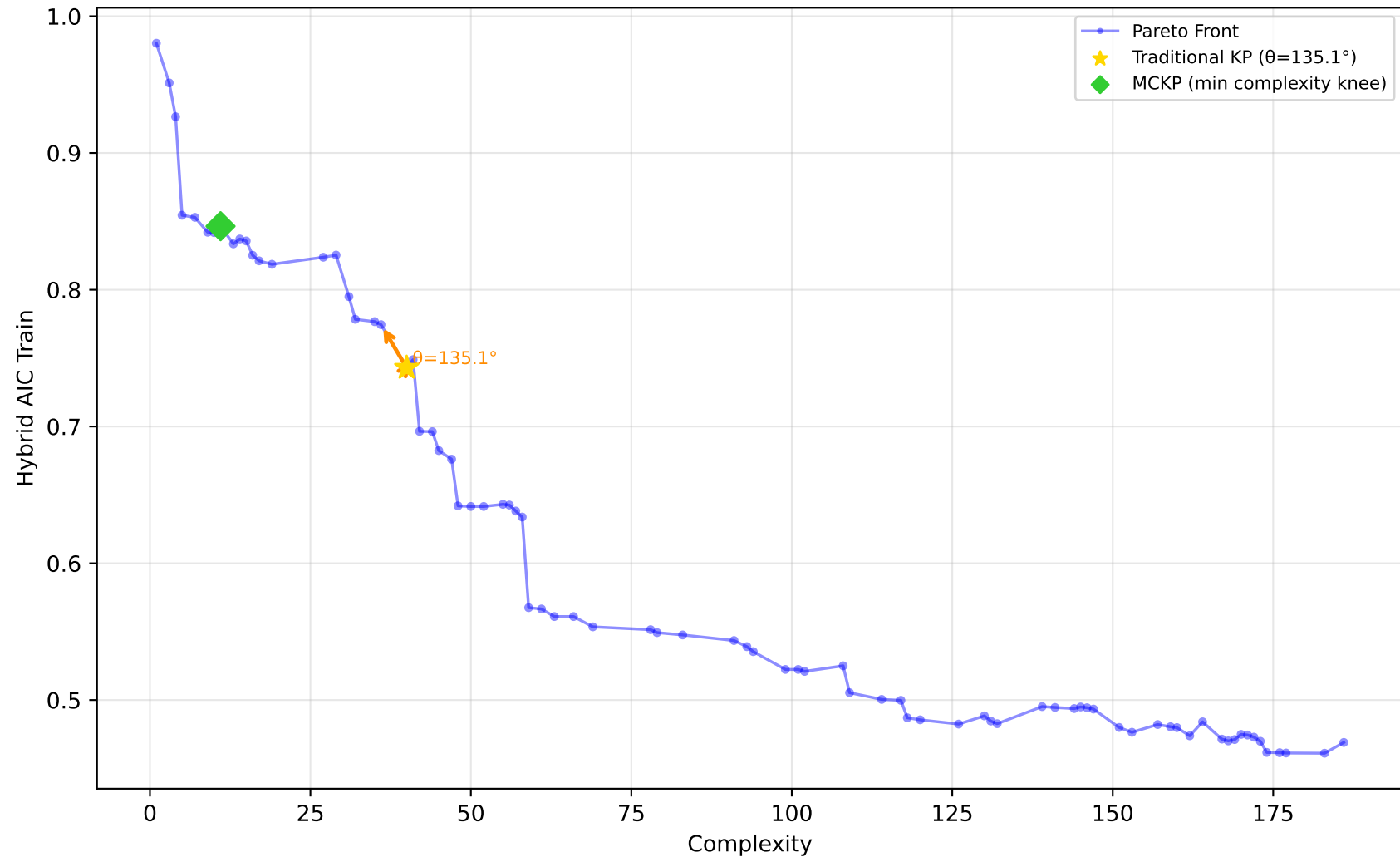
1096_FacultySalaries - Run 18 - MVP - Hybrid AIC Train \lambda_1=0.10, \lambda_2=0.00, \lambda_3=0.00 | Difficulty: 1.00 | Method: hmr
