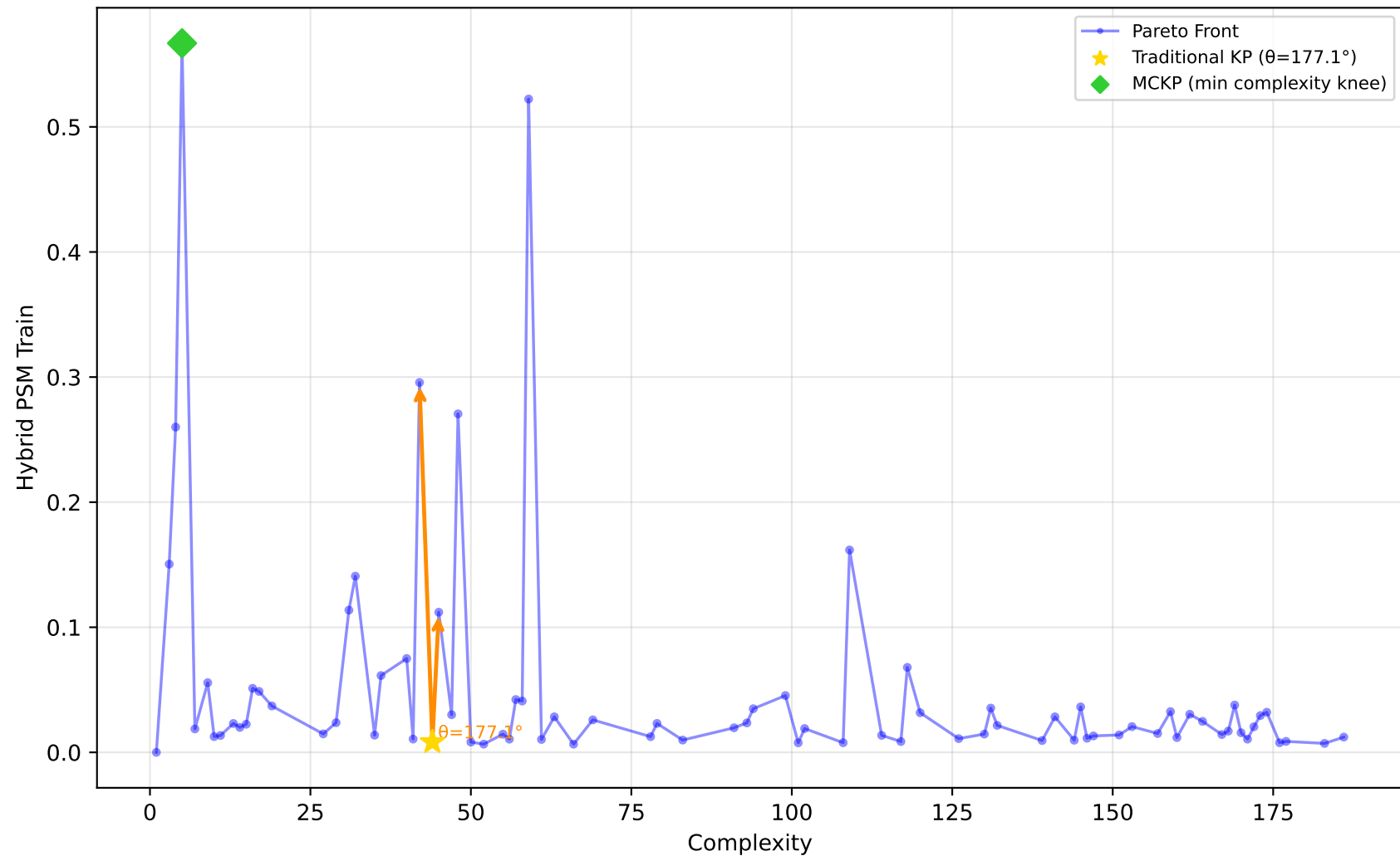
1096_FacultySalaries - Run 18 - MVP - Hybrid PSM Train \lambda_1=0.10, \lambda_2=0.00, \lambda_3=0.00 | Difficulty: 1.00 | Method: hmr
