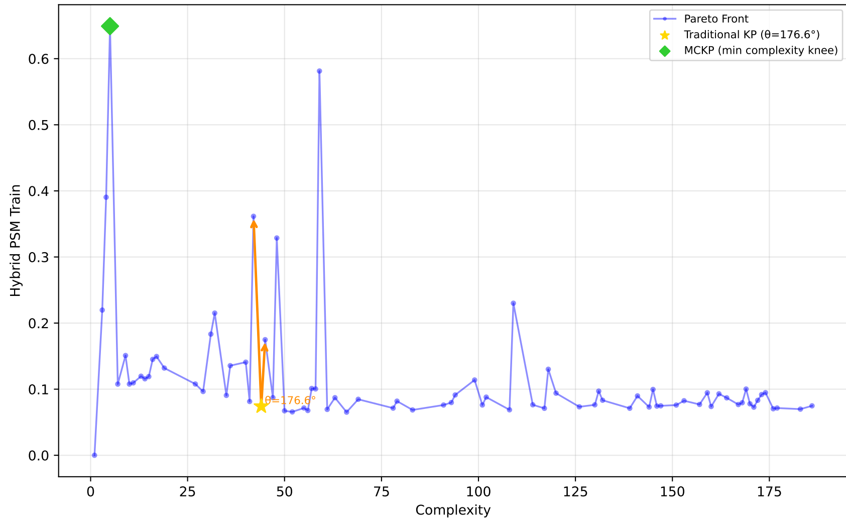
1096_FacultySalaries - Run 18 - MVP - Hybrid PSM Train \lambda_1=1.00, \lambda_2=0.00, \lambda_3=0.00 | Difficulty: 1.00 | Method: hmr
